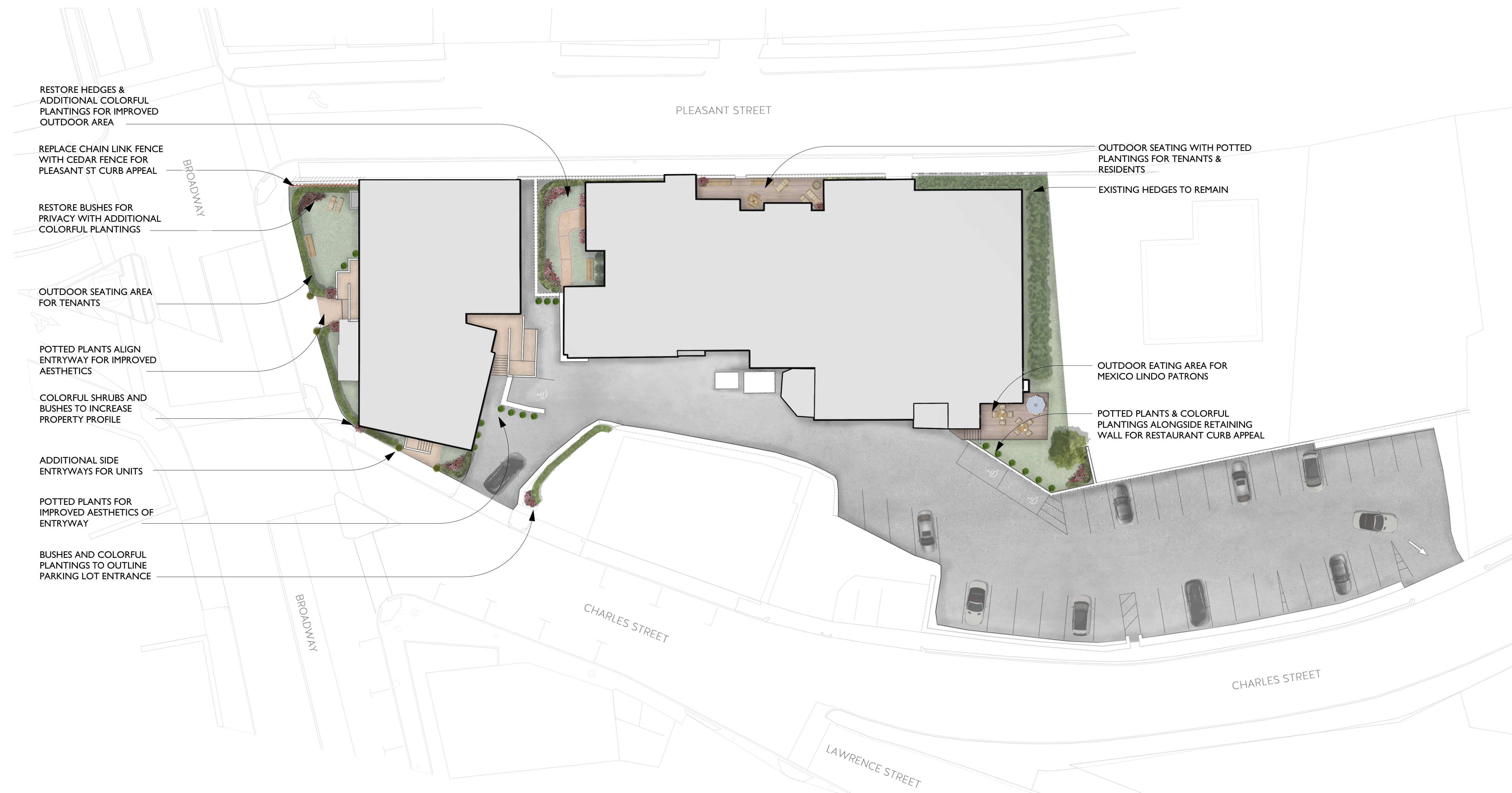
1 LANDSCAPE PLAN
